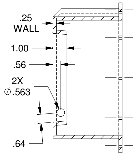
SECTION J-J
